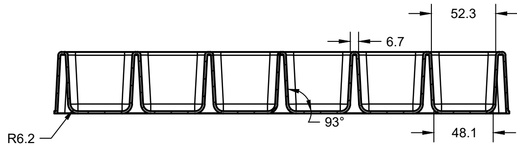
SECTION B-B SCALE 1:3
